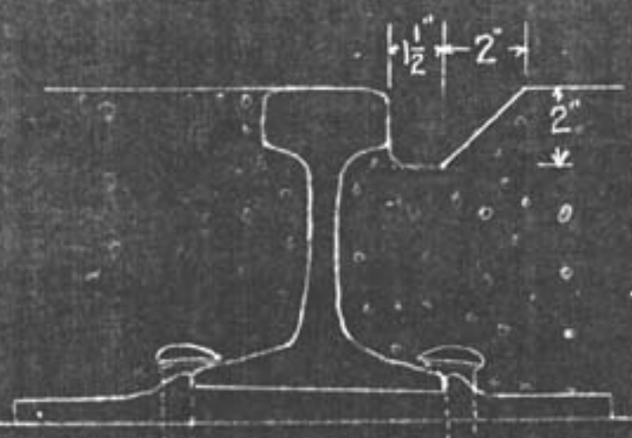
Sketch Showing Flangeway.
